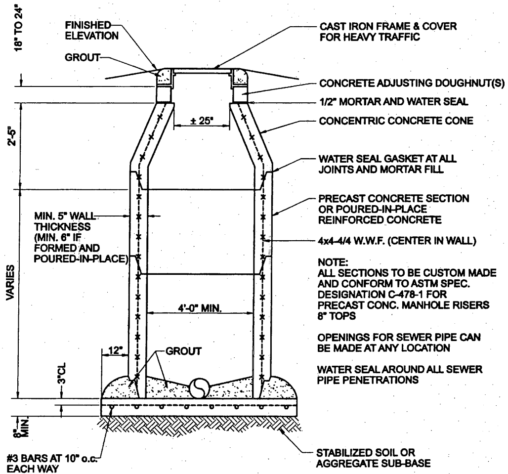
Typical Sewer Manhole Figure 13
