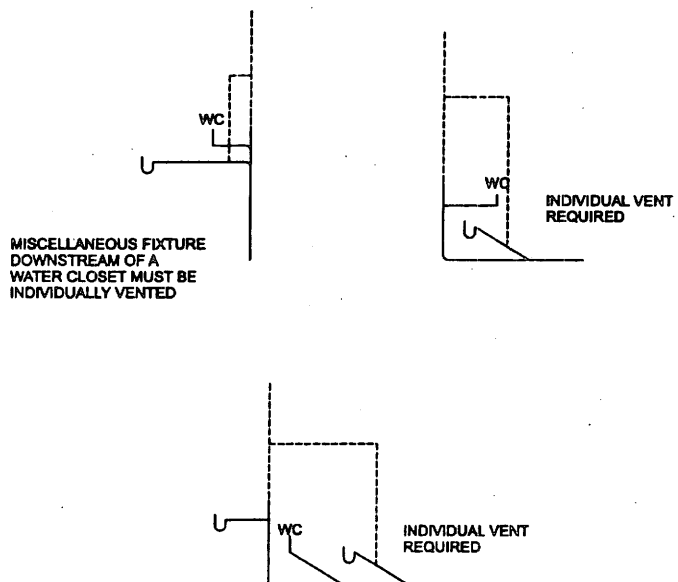
Required Individual Vents Figure 9-41
