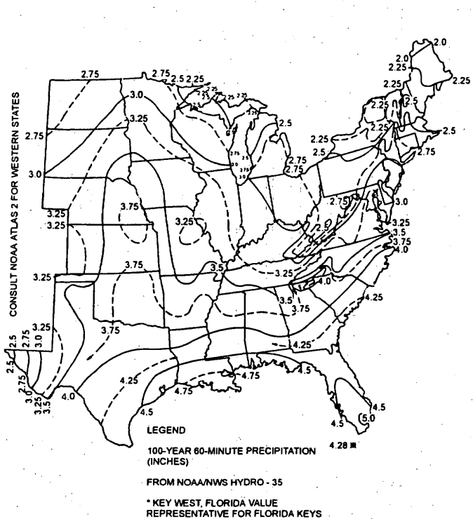
FIGURE 1108.4 RAINFALL RATES FOR PRIMARY ROOF DRAINS (IN/HR)
