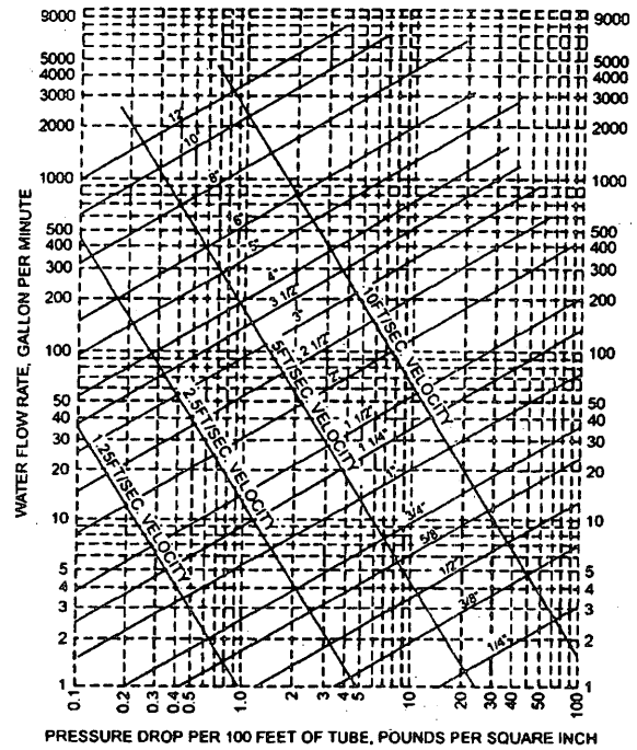
Figure F103A.2 Friction Loss in Smooth Pipe 1 (Type L, ASTM B88 Copper Tubing)
