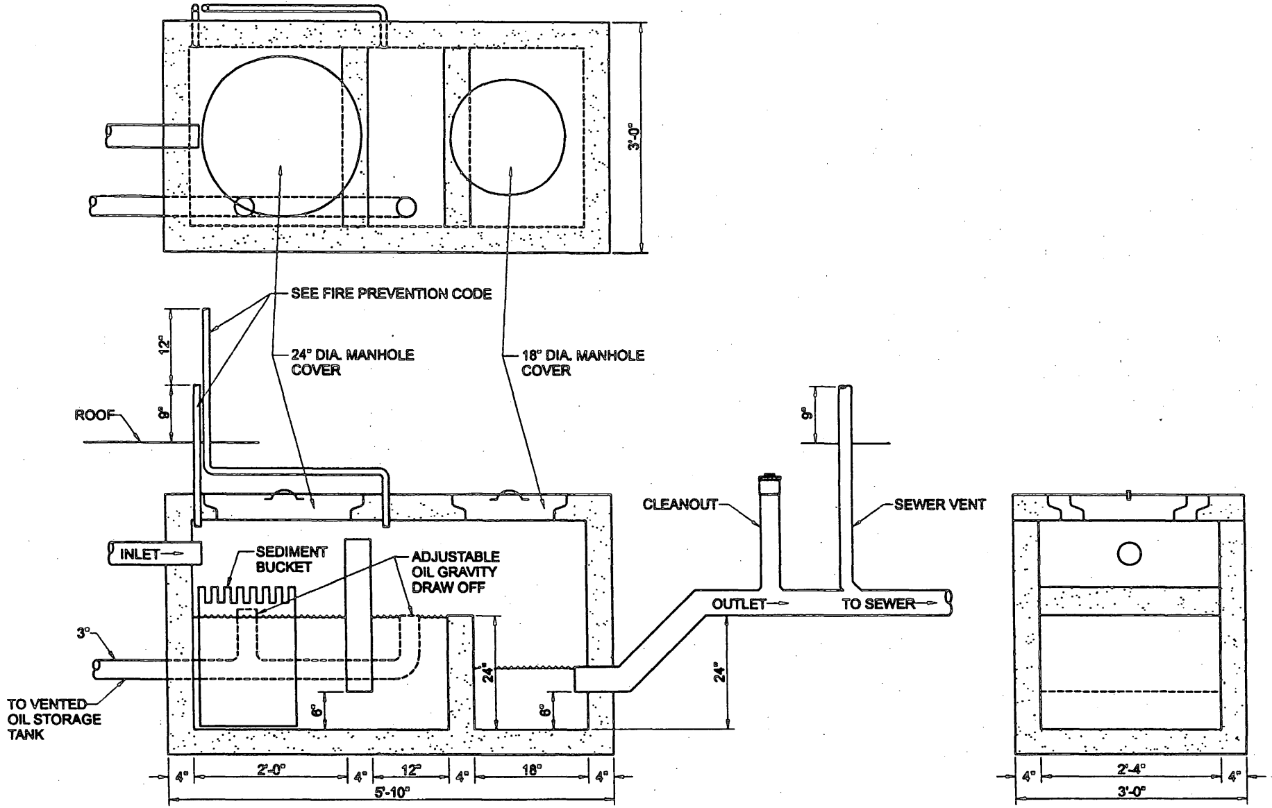
Oil Interceptor Details Figure M106.B
